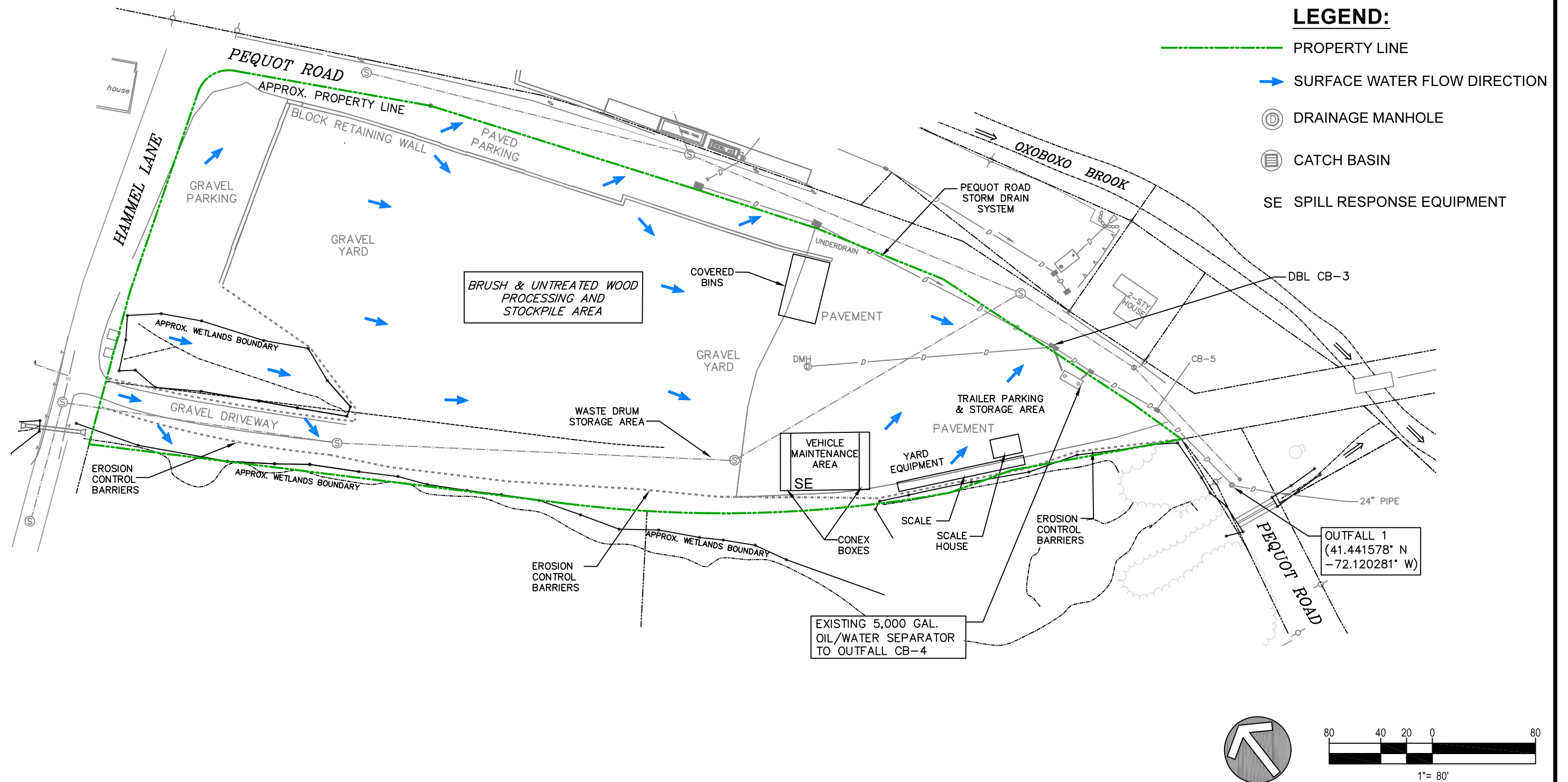
FIGURE 2: SITE PLAN
